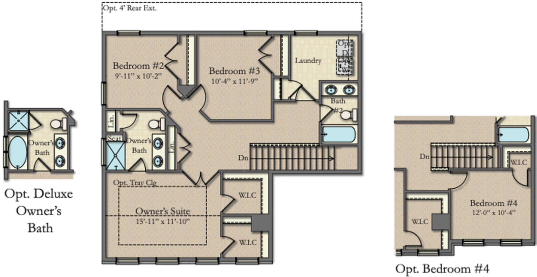
ALT. SECOND FLOOR
