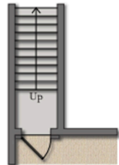
Full Straight Areaway
